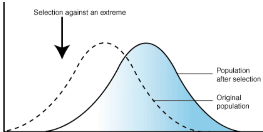
Figure%: The effect of directional selection on trait distribution
