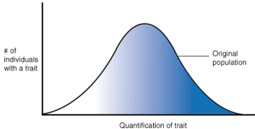
Figure%: The standard distribution of a trait across a population
