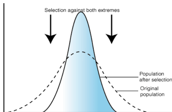
Figure%: The effect of stabilizing selection on trait distribution
