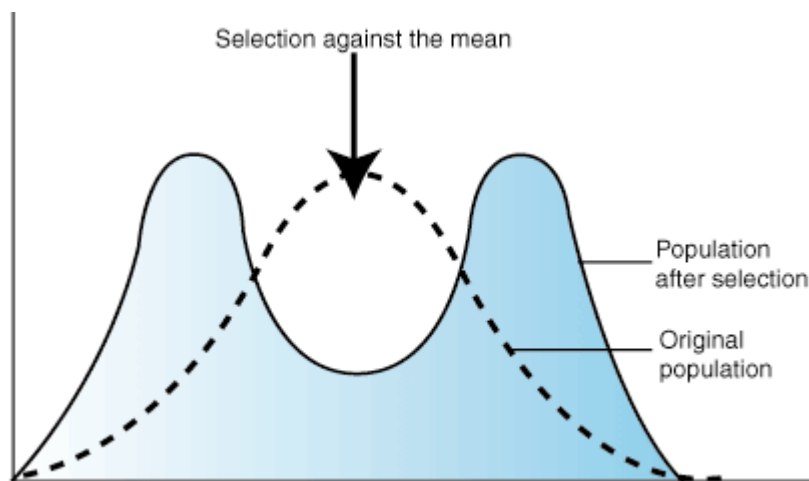
Figure%: The effect of disruptive selection on trait distribution
